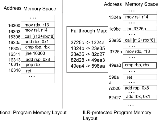
Figure 9: Instruction location randomization. This figure is adopted from ILR [52].
